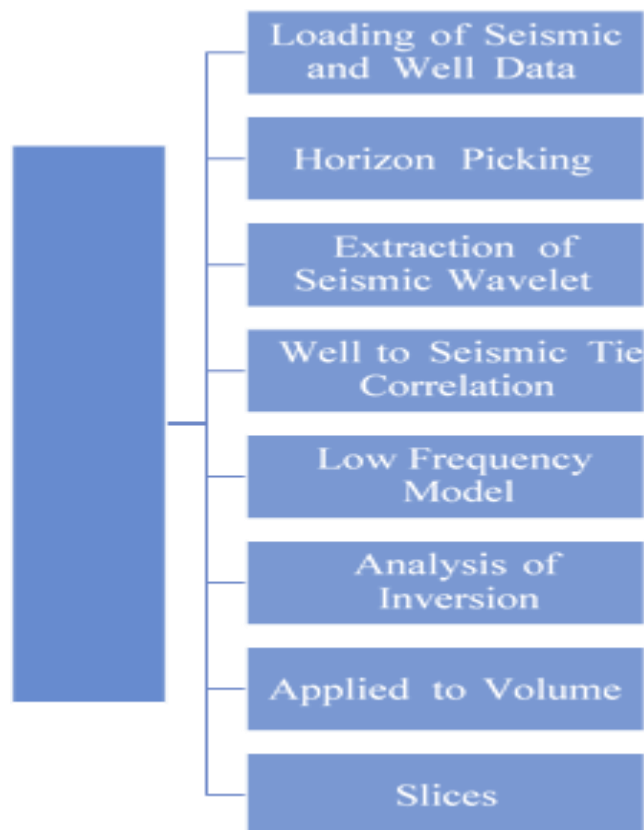
Figure 6.2: Workflow Adopted for Modal Based Inversion
