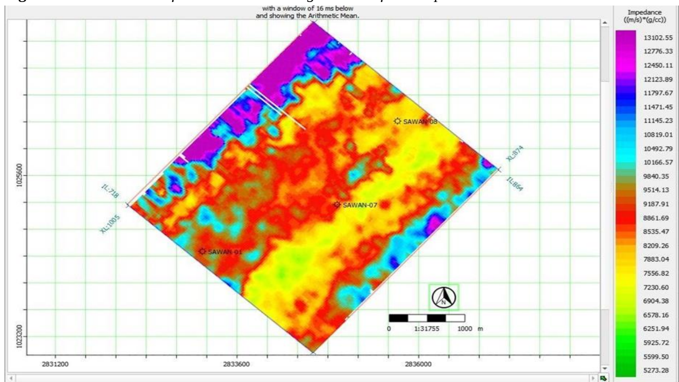
Figure 6.7: 3D cube slice for C Interval showing variation for P-Impedance.
