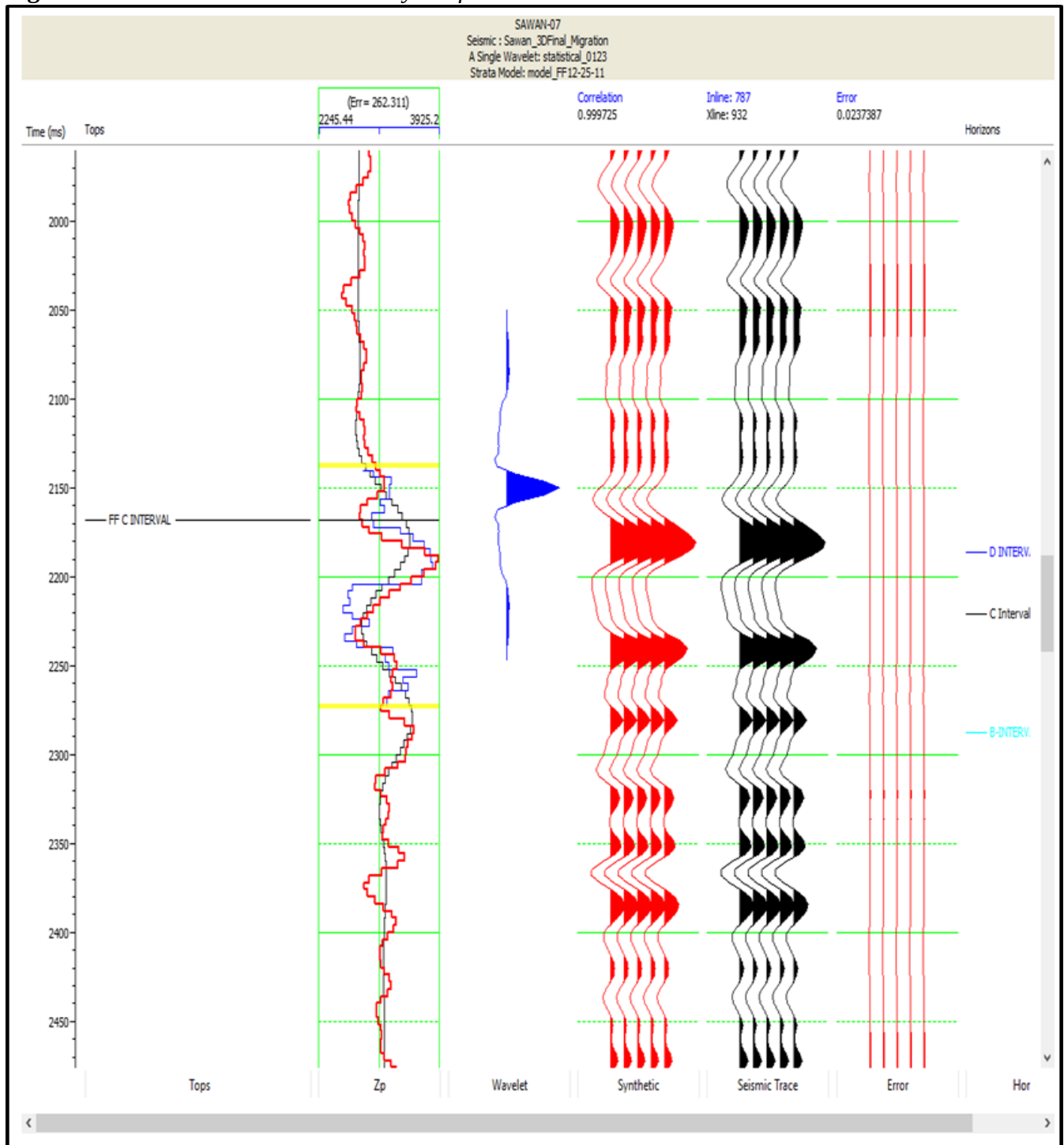
Figure 6.5: Model based inversion analysis of Sawan-07
